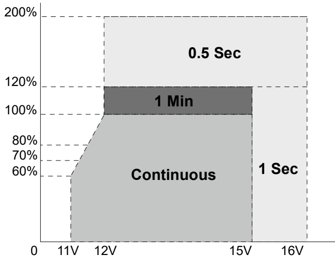
Figure 1 : Output power VS input voltage
